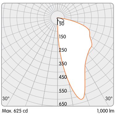
Stealth Reflector
